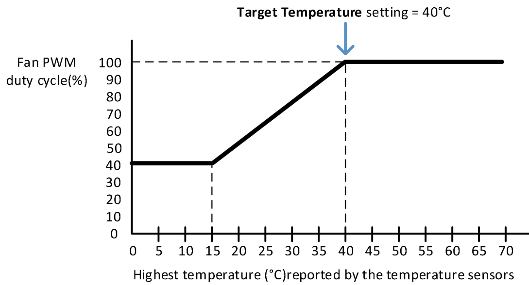
Figure 32 Change Target Temperature to 40°C
